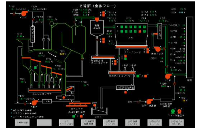
CRT
