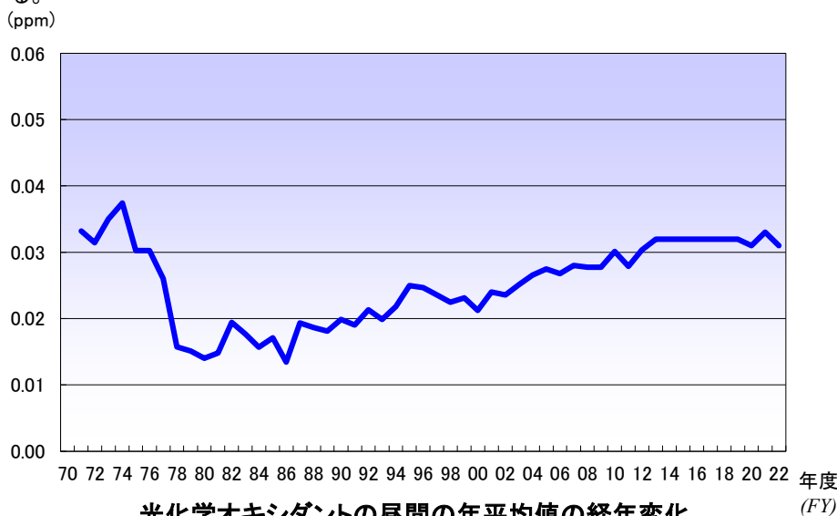
光化学オキシダントの昼間の年平均値の経年変化 (A Long-Term Trend of Annual Average Ox Concentration during the Daytime)
