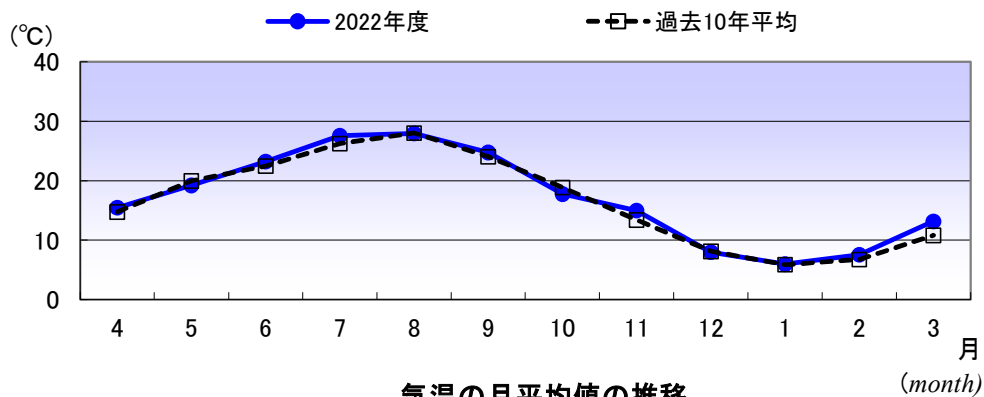
気温の月平均値の推移 (Trend of Monthly Average of TEMP) <図9-3>
