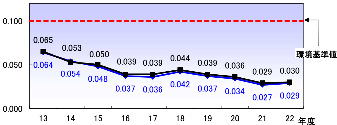
浮遊粒子状物質の日平均値の2%除外値の推移(過去10年間) (Trend of 2%-excluded Value of Daily Average SPM Concentration (The Last Ten Years))
