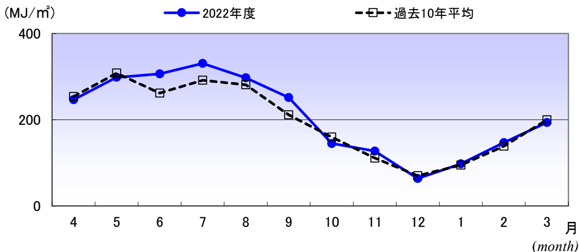
放射収支量の月合計値の平均の推移 (Trend of Total Monthly Amount of Radiation Balance) <図9-7>
