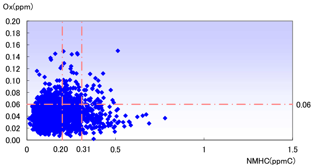
NMHCの3時間平均値とOxの昼間の1時間値の最高値の関係(2022年度) (Relationship between 3-hour Average NMHC Concentration and Maximum Ox Concentration during the Daytime : FY2022)
