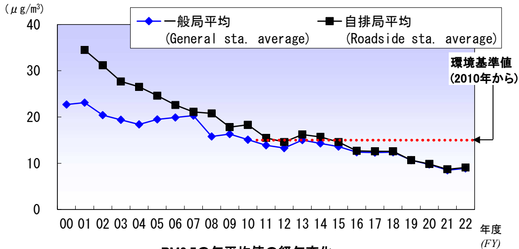
PM2.5の年平均値の経年変化 (A Long-Term Trend of Annual Average PM2.5 Concentration)
